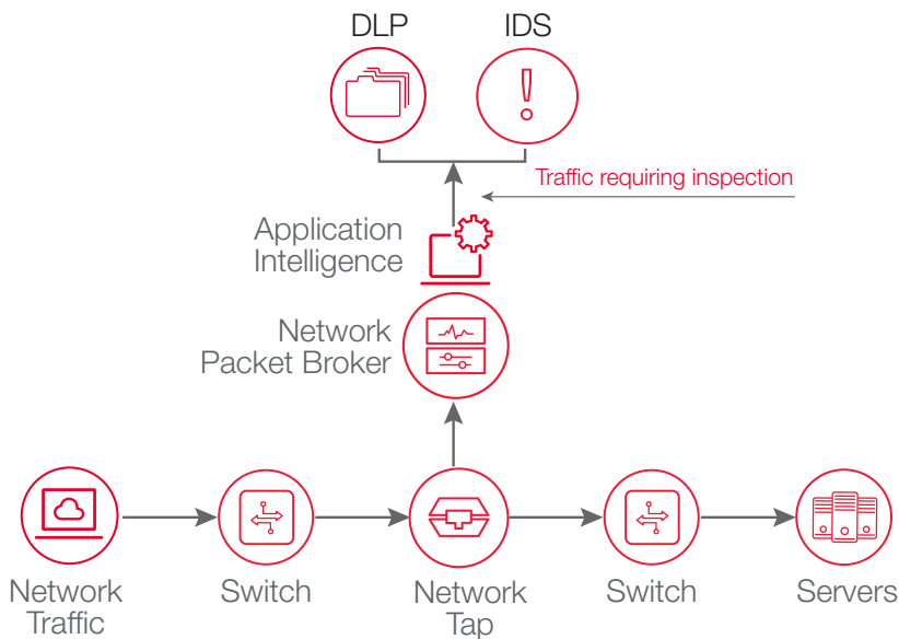
Figure 6. Step 6: Enable deep packet inspection.
