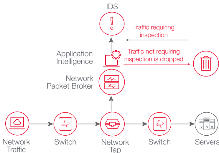
Figure 5. Step 5: Perform advanced data filtering to remove low threat data.
