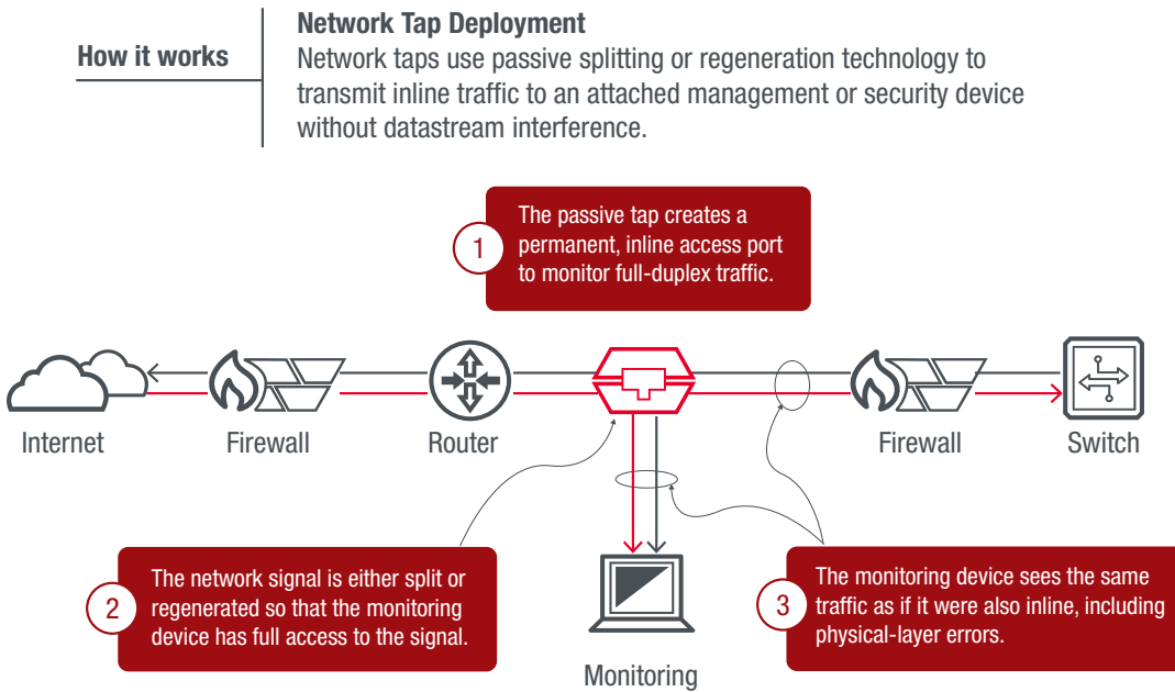
Figure 1. Network Tap Deployment
